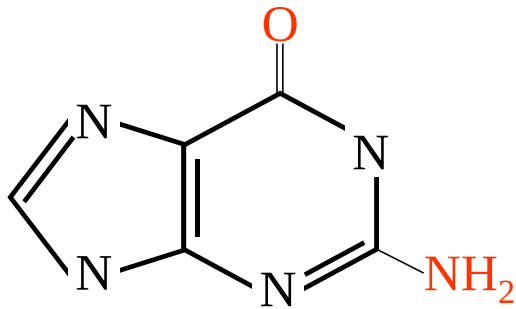
GUANİN
