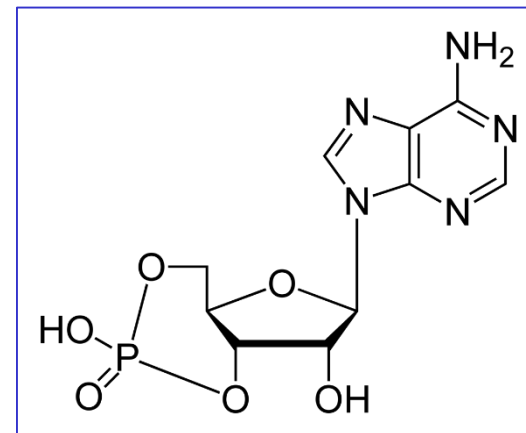
cAMP
